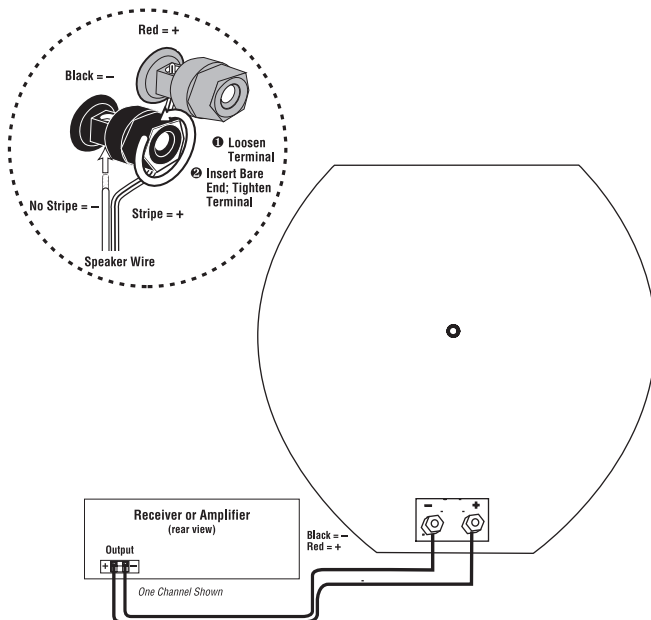
Figure 4. Wiring diagram shows polarity connections for one channel of a home theater system.
